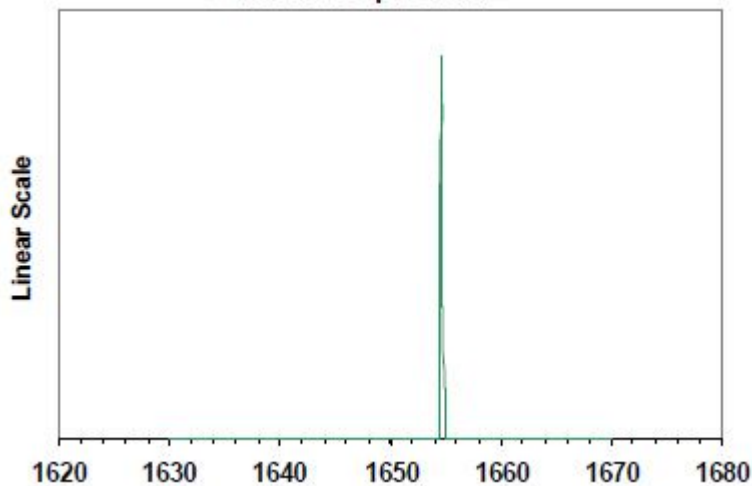
Emission Spectrum
